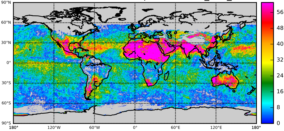
MCDC OBS NOBS: AOD - Experiment nnr_003_c061
