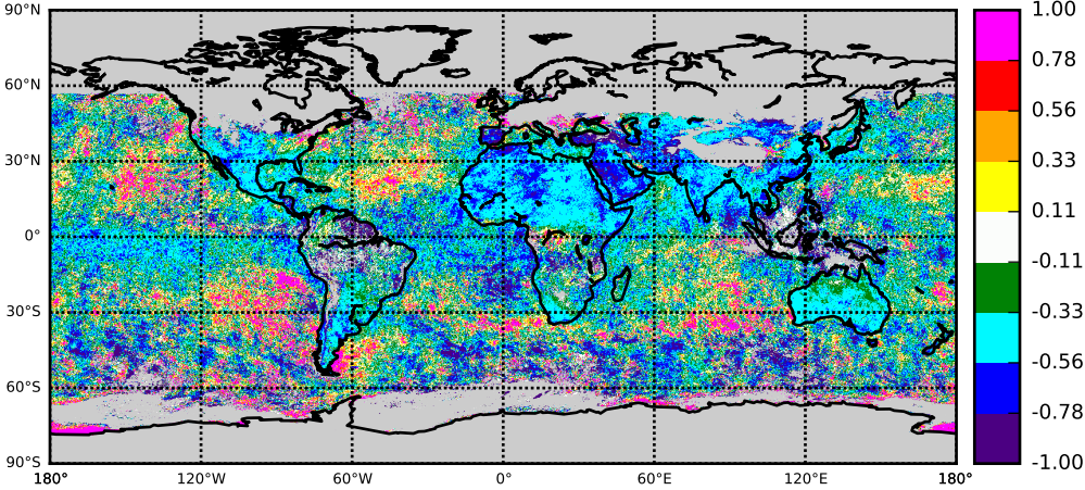
MCDC OBS NOBS: TOP minus MIDDLE/MIDDLE
