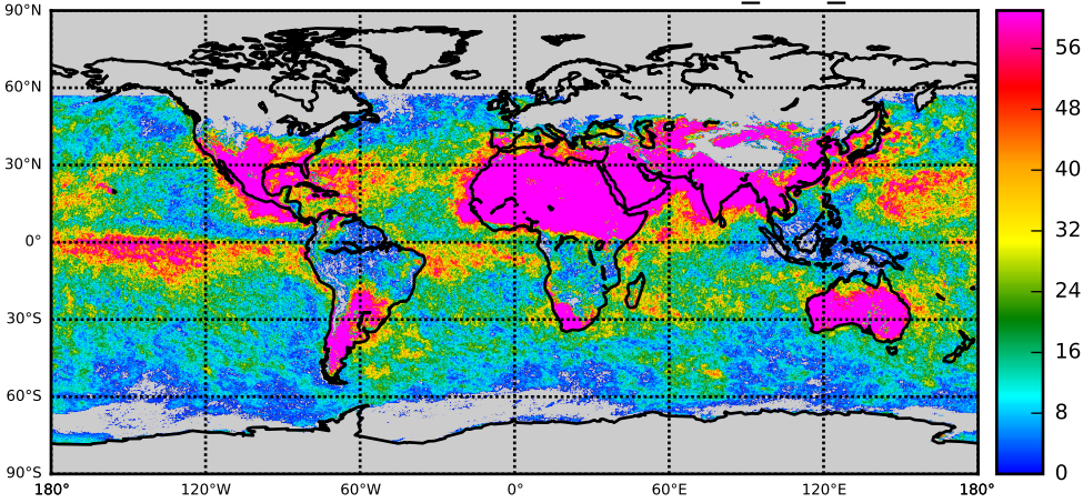
MCDC OBS NOBS: AOD - Control nnr_003_c006
