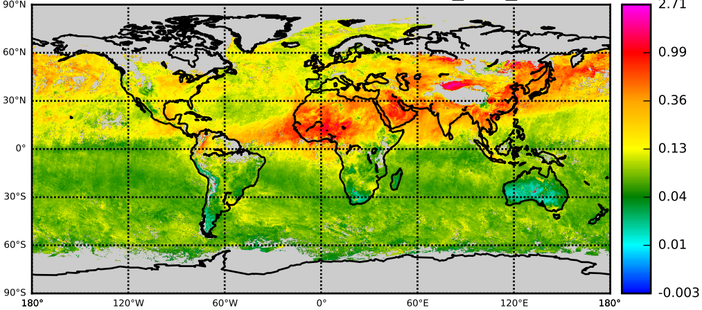
MODC OBS: AOD - Experiment nnr_003_c061
