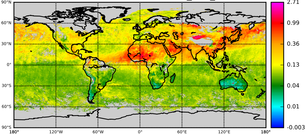
MODC OBS: AOD - Control nnr_003_c006
