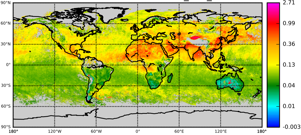
MODC OBS: AOD - Control nnr_003_c006
