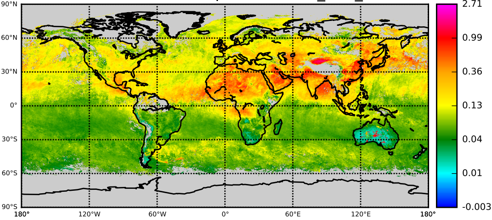
MODC OBS: AOD - Experiment nnr_003_c061
