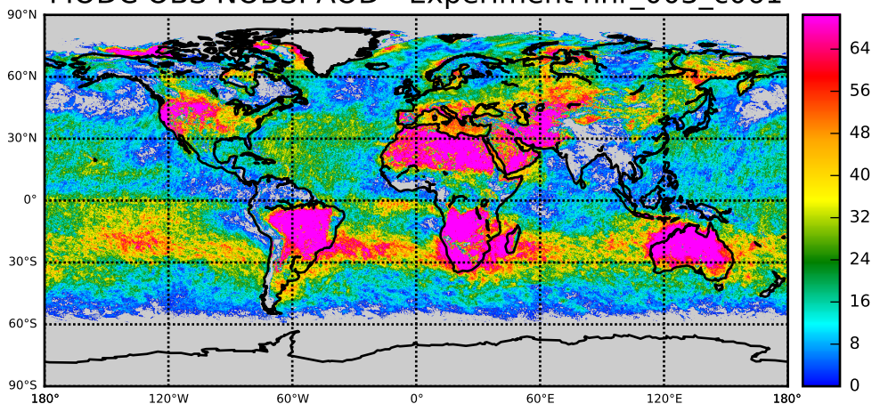
MODC OBS NOBS: AOD - Experiment nnr_003_c061
