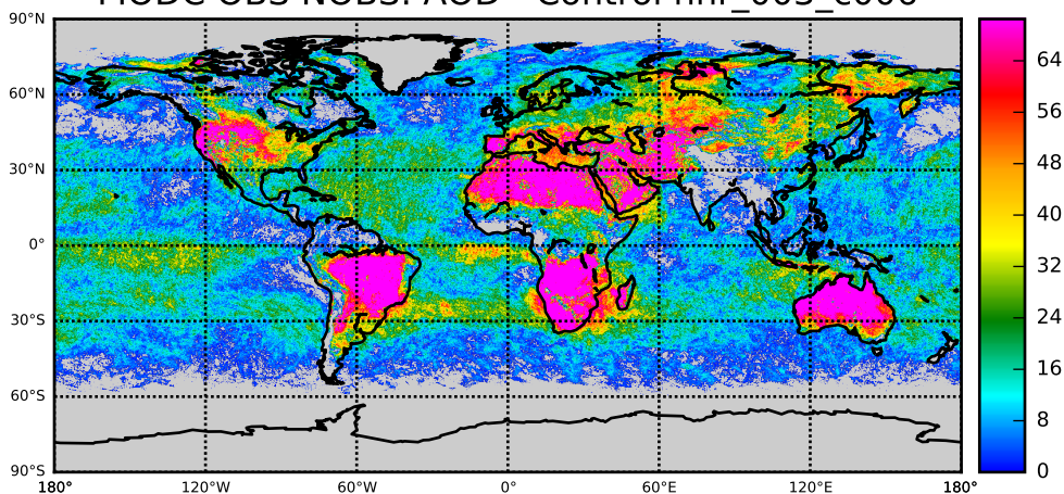
MODC OBS NOBS: AOD - Control nnr_003_c006
