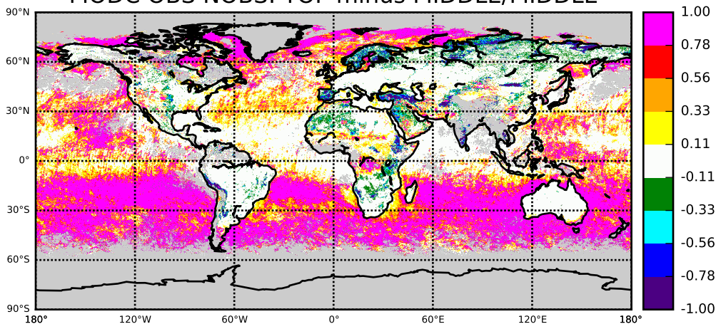
MODC OBS NOBS: TOP minus MIDDLE/MIDDLE
