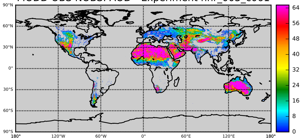
MODD OBS NOBS: AOD - Experiment nnr_003_c061
