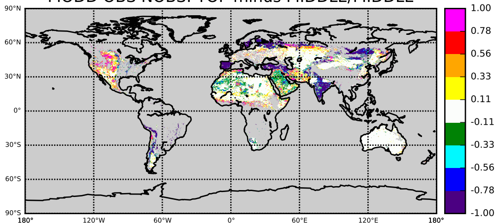
MODD OBS NOBS: TOP minus MIDDLE/MIDDLE
