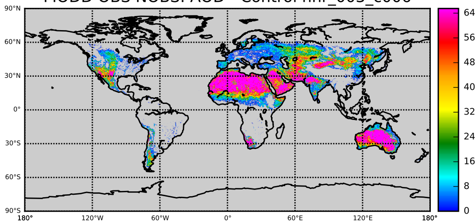
MODD OBS NOBS: AOD - Control nnr_003_c006
