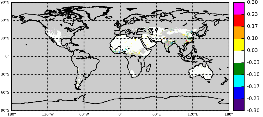
MODD OBS: TOP minus MIDDLE
