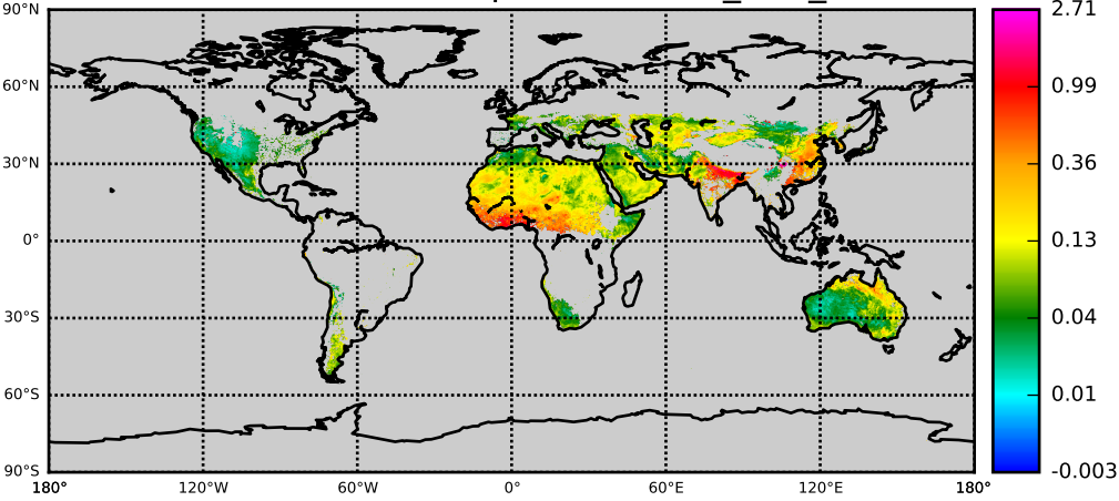
MODD OBS: AOD - Experiment nnr_003_c061
