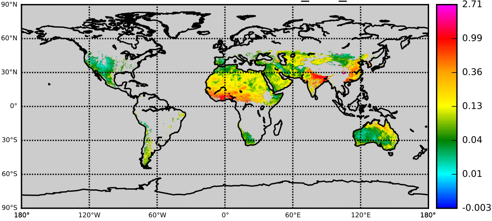
MODD OBS: AOD - Control nnr_003_c006
