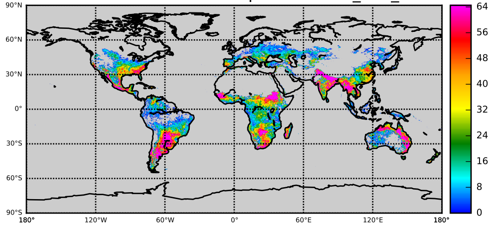
MODL OBS NOBS: AOD - Experiment nnr_003_c061
