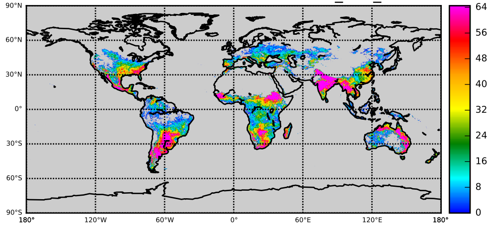
MODL OBS NOBS: AOD - Control nnr_003_c006
