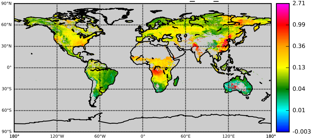
MODL OBS: AOD - Control nnr_003_c006
