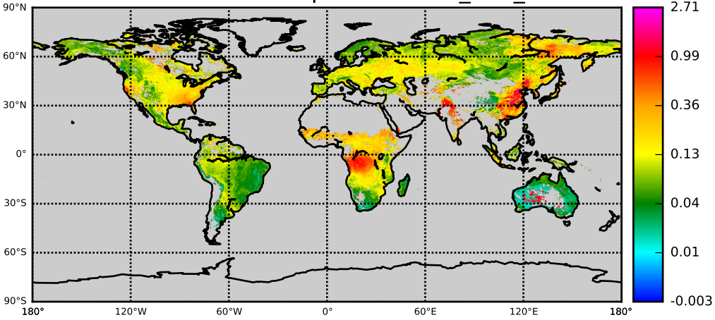
MODL OBS: AOD - Experiment nnr_003_c061
