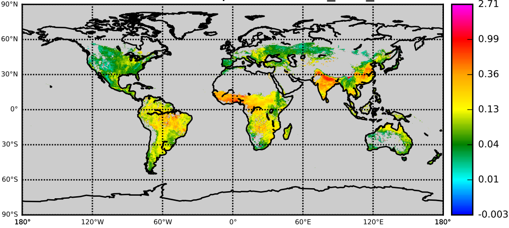
MODL OBS: AOD - Experiment nnr_003_c061
