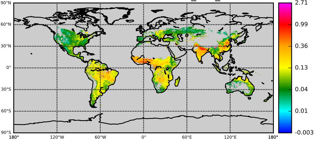
MODL OBS: AOD - Control nnr_003_c006
