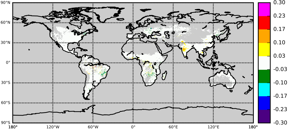
MODL OBS: TOP minus MIDDLE
