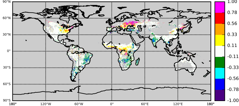
MODL OBS NOBS: TOP minus MIDDLE/MIDDLE
