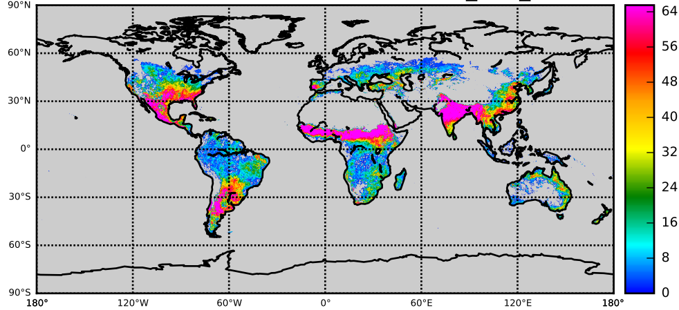
MODL OBS NOBS: AOD - Control nnr_003_c006
