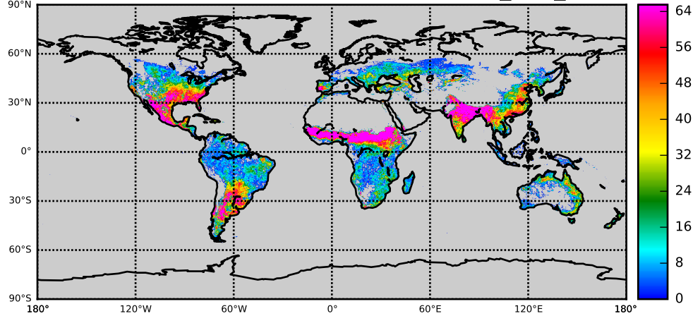
MODL OBS NOBS: AOD - Experiment nnr_003_c061
