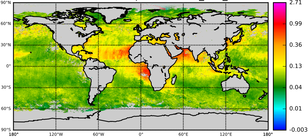
MOD0 OBS: AOD - Experiment nnr_003_c061
