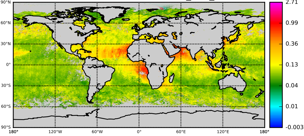
MOD0 OBS: AOD - Control nnr_003_c006
