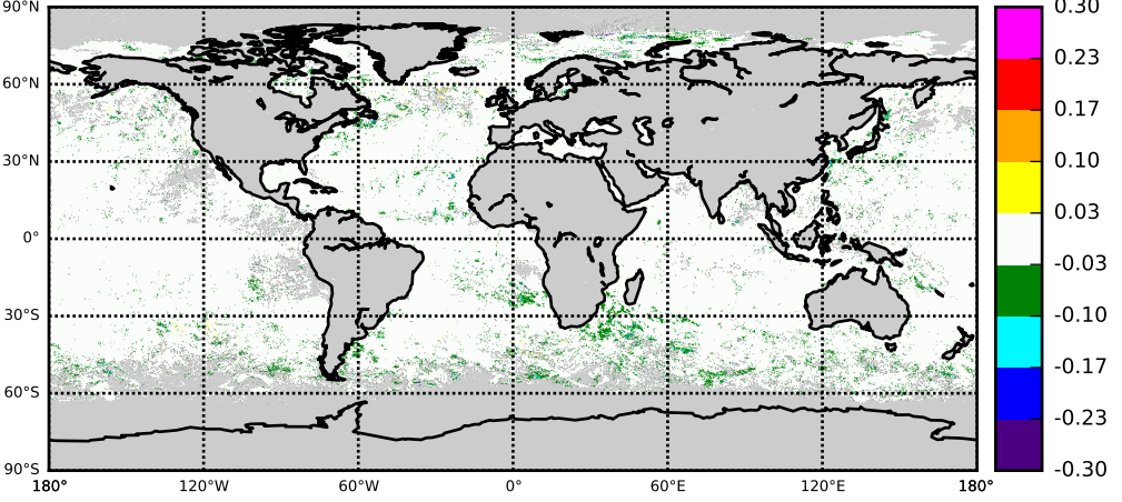
MOD0 OBS: TOP minus MIDDLE
