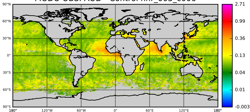
MOD0 OBS: AOD - Control nnr_003_c006
