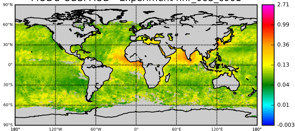
MOD0 OBS: AOD - Experiment nnr_003_c061
