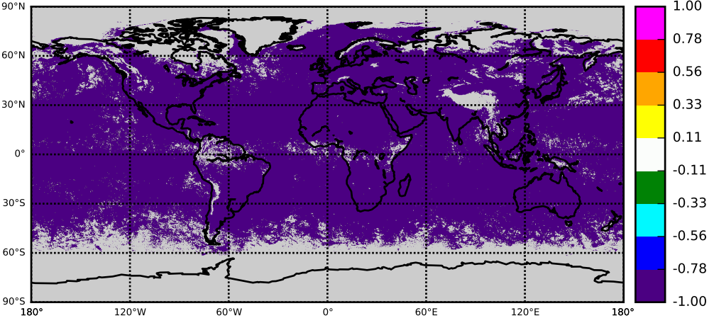
MYDC OBS NOBS: TOP minus MIDDLE/MIDDLE
