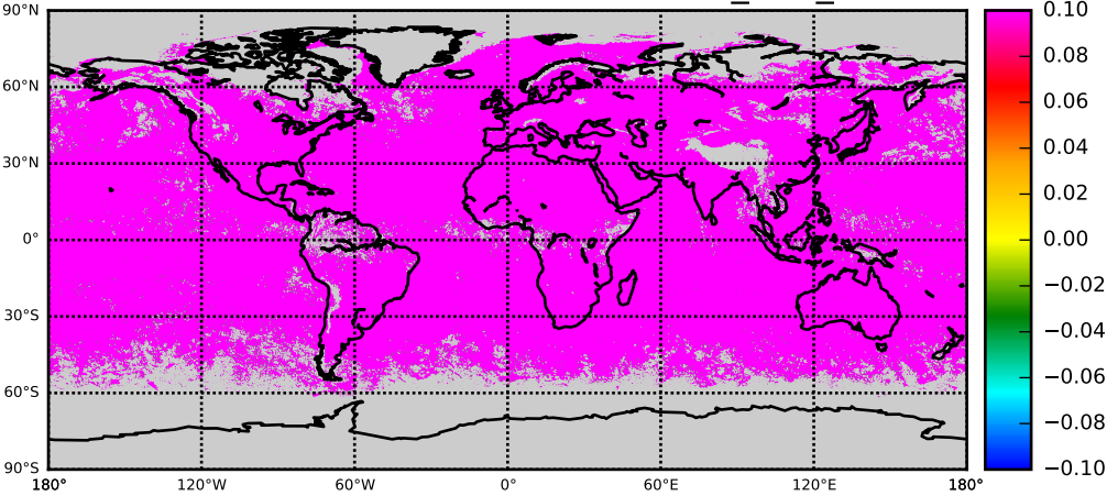
MYDC OBS NOBS: AOD - Control nnr_003_c006
