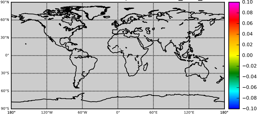
MYDC OBS NOBS: AOD - Experiment nnr_003_c061
