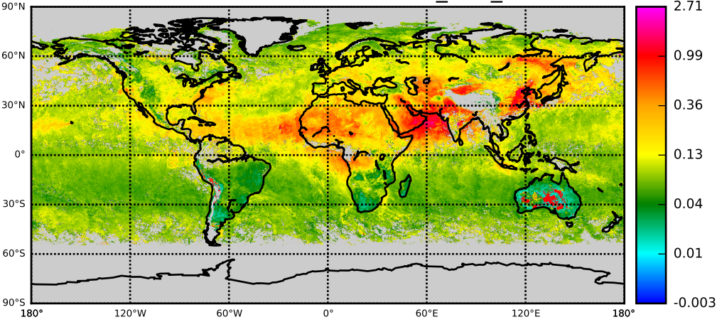
MYDC OBS: AOD - Control nnr_003_c006
