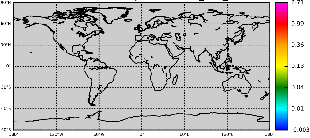
MYDC OBS: AOD - Experiment nnr_003_c061
