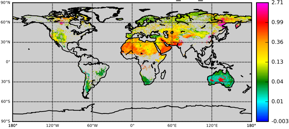
MYDD OBS: AOD - Control nnr_003_c006
