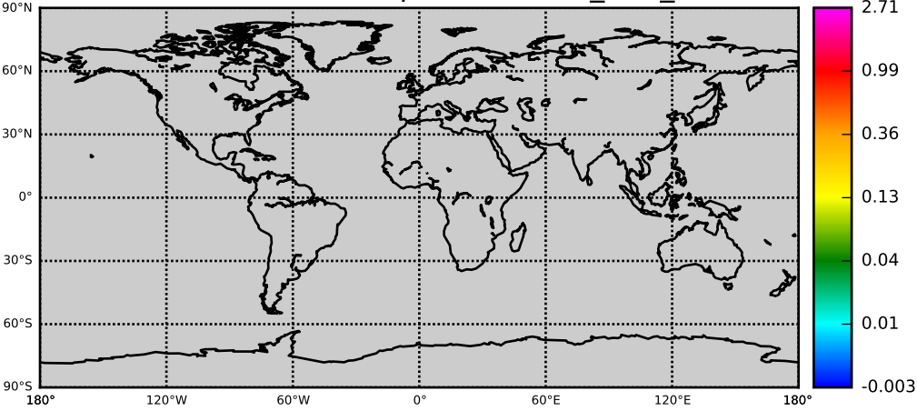
MYDD OBS: AOD - Experiment nnr_003_c061
