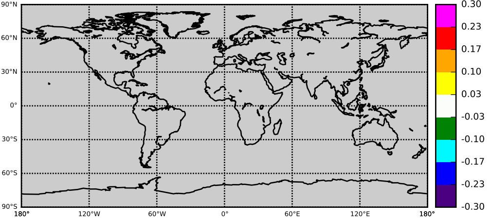
MYDL OBS: TOP minus MIDDLE
