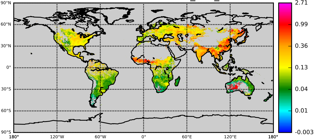
MYDL OBS: AOD - Control nnr_003_c006
