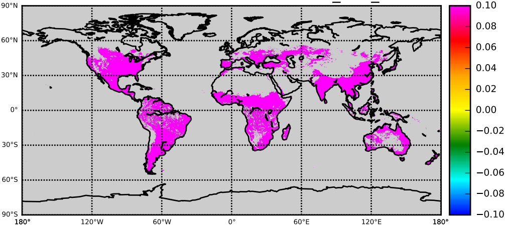
MYDL OBS NOBS: AOD - Control nnr_003_c006
