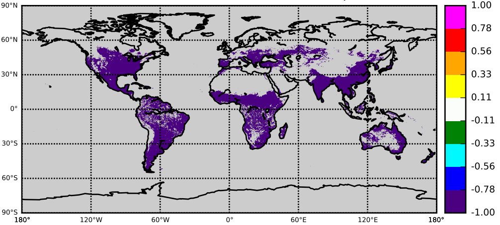
MYDL OBS NOBS: TOP minus MIDDLE/MIDDLE
