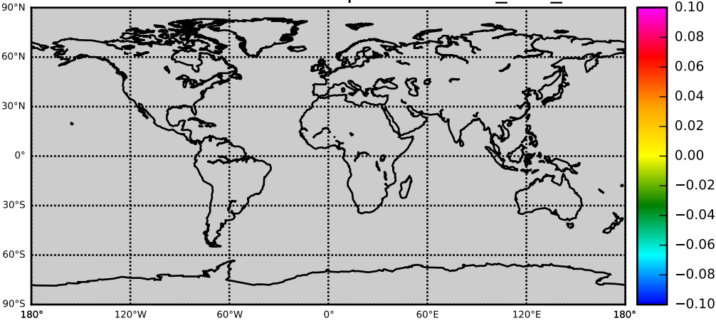
MYDL OBS NOBS: AOD - Experiment nnr_003_c061
