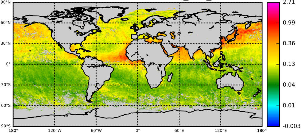
MYDO OBS: AOD - Control nnr_003_c006
