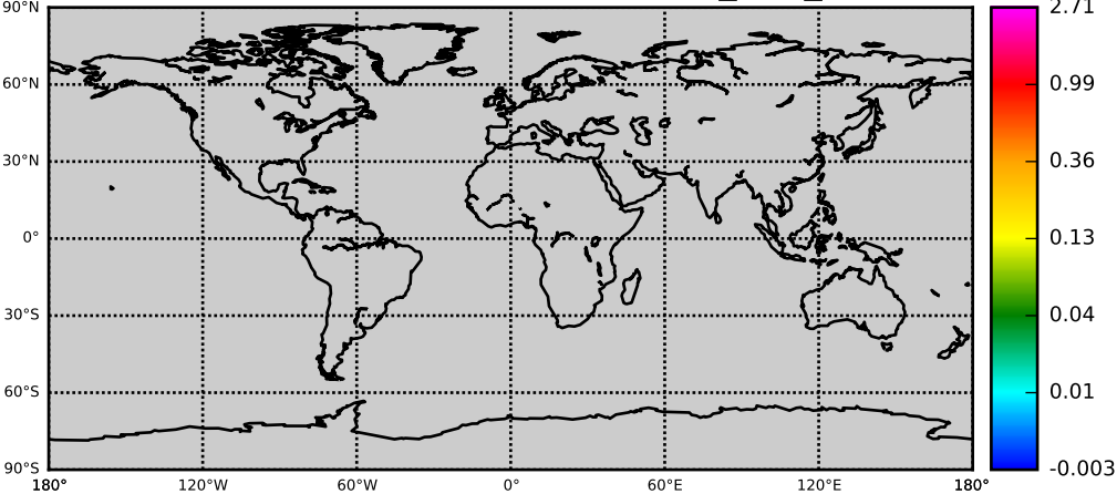
MYDO OBS: AOD - Experiment nnr_003_c061
