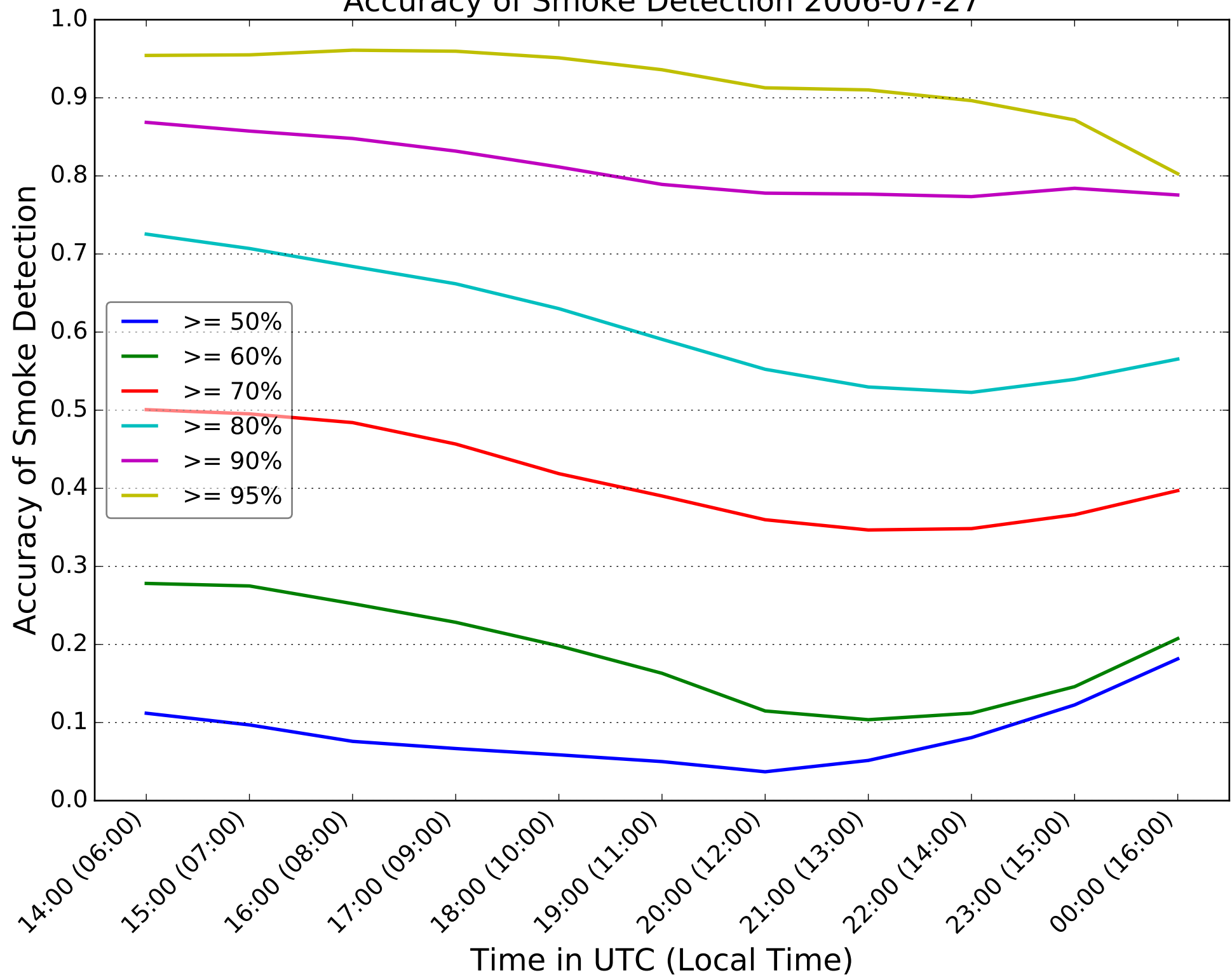
Accuracy of Smoke Detection 2006-07-27
