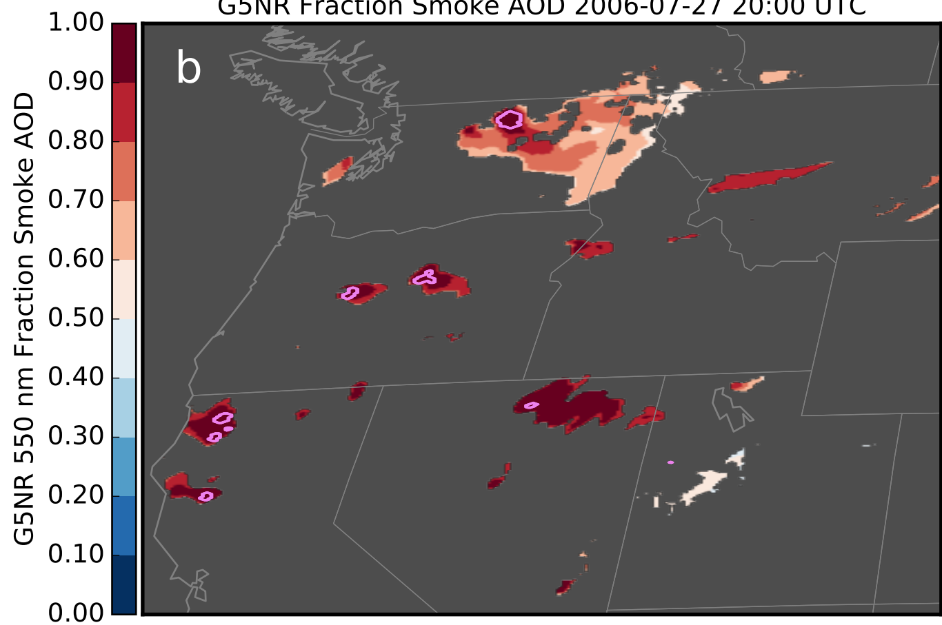
G5NR Fraction Smoke AOD 2006-07-27 20:00 UTC
