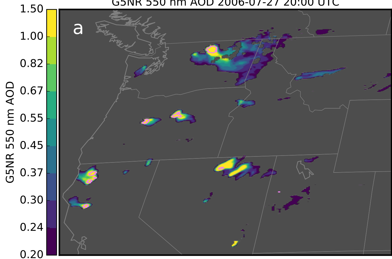
G5NR 550 nm AOD 2006-07-27 20:00 UTC
