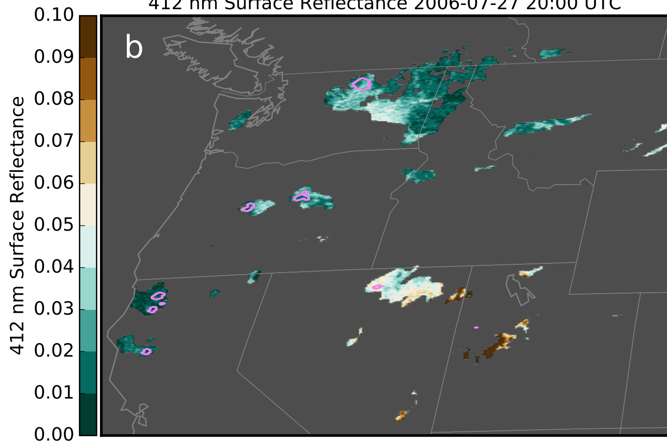
412 nm Surface Reflectance 2006-07-27 20:00 UTC
