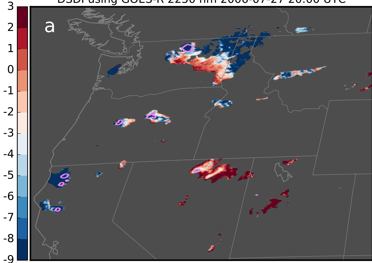
DSDI using GOES-R 2250 nm 2006-07-27 20:00 UTC
