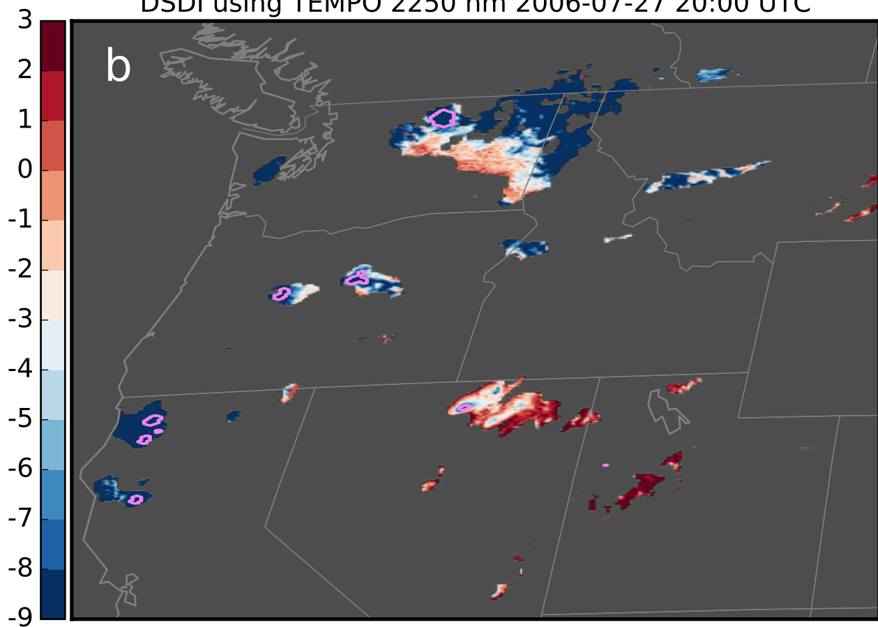
DSDI using TEMPO 2250 nm 2006-07-27 20:00 UTC
